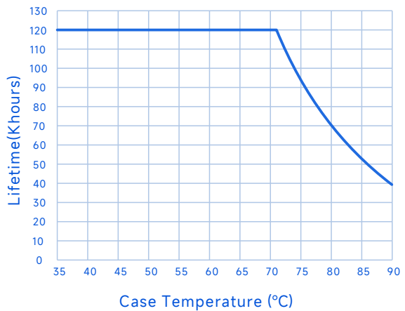
Lifespan vs. Case Temperature
