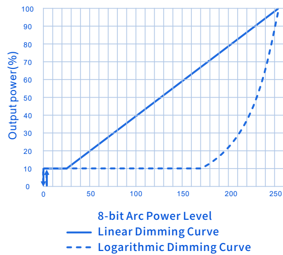
Linear and Logarithmic Dimming Curves
